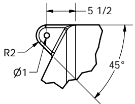
DETAIL B SCALE 1 / 12
