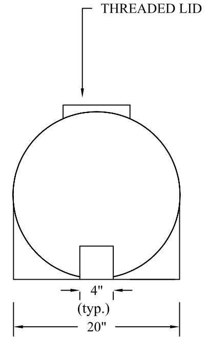
END VIEW
